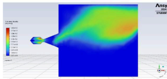
Fig.10. Turbulent viscosity
